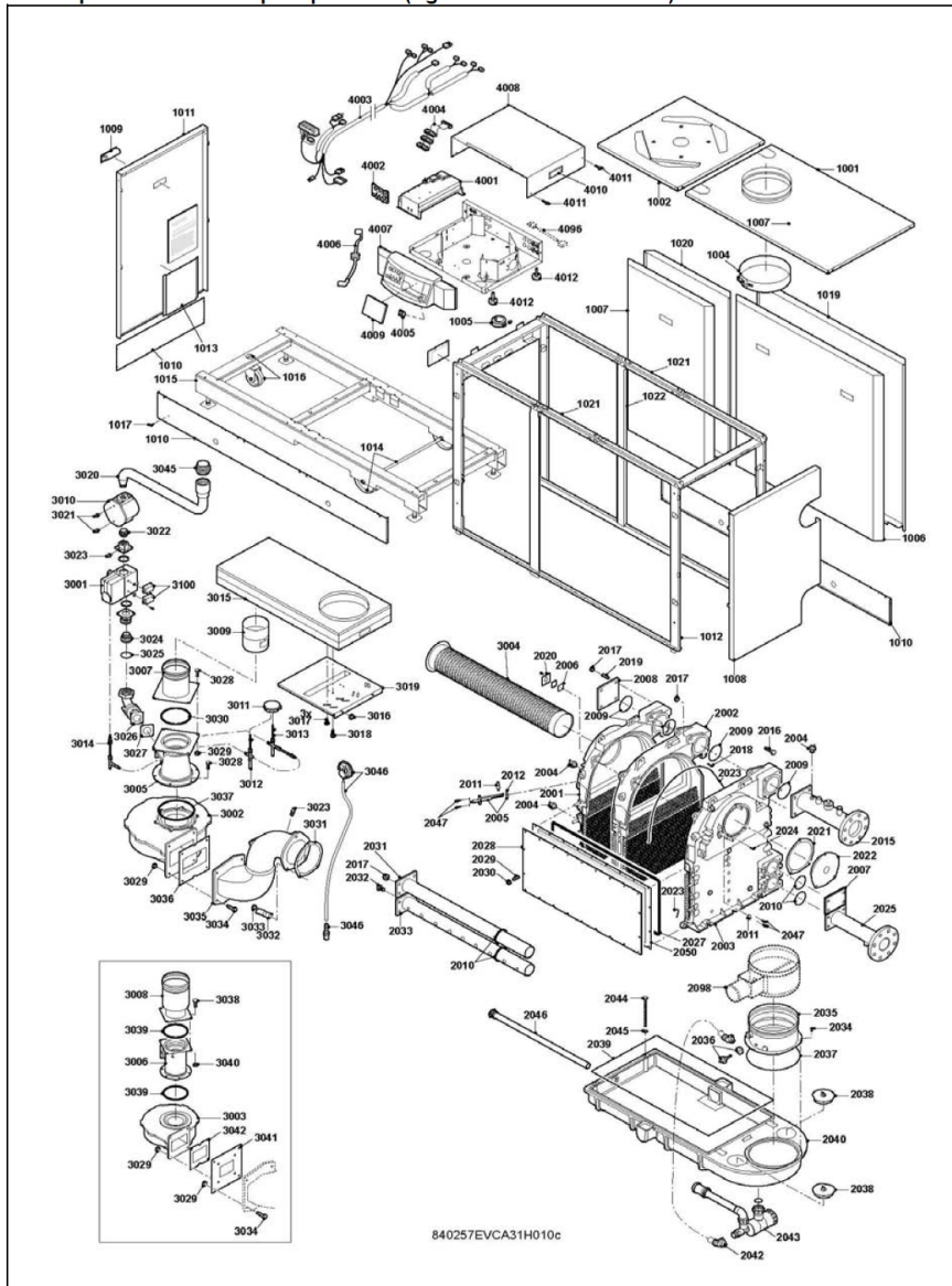
15.5 Exploded view and spare parts list (right hand version shown)
